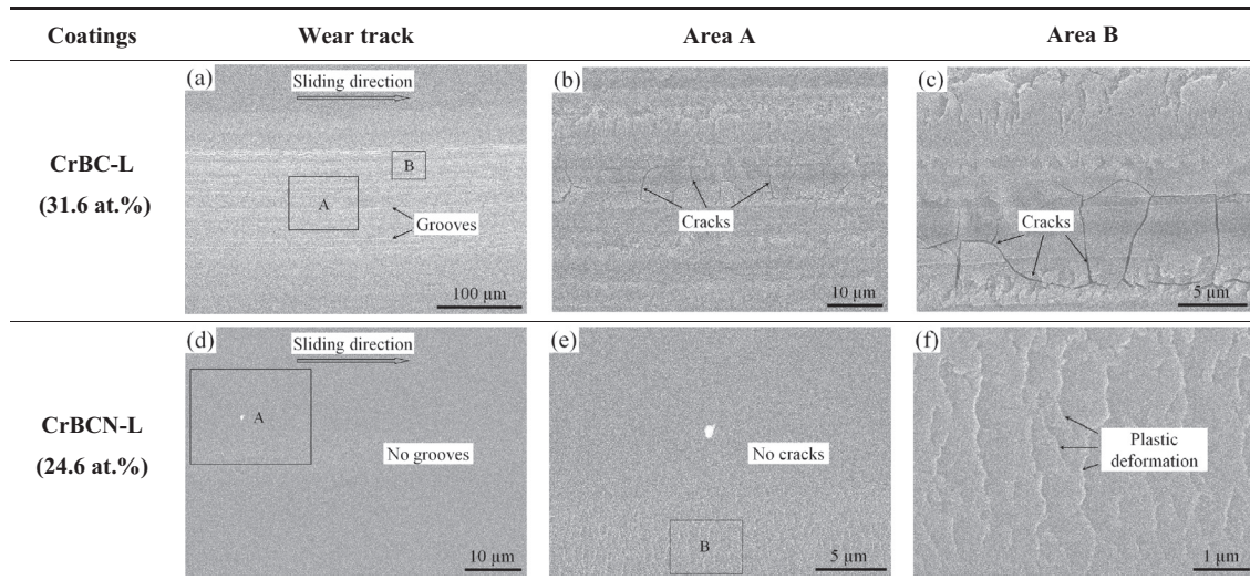
Fig. 9. SEM images of wear tracks on (a) (b) (c) CrBC-L and (d) (e) (f) CrBCN-L coatings.
