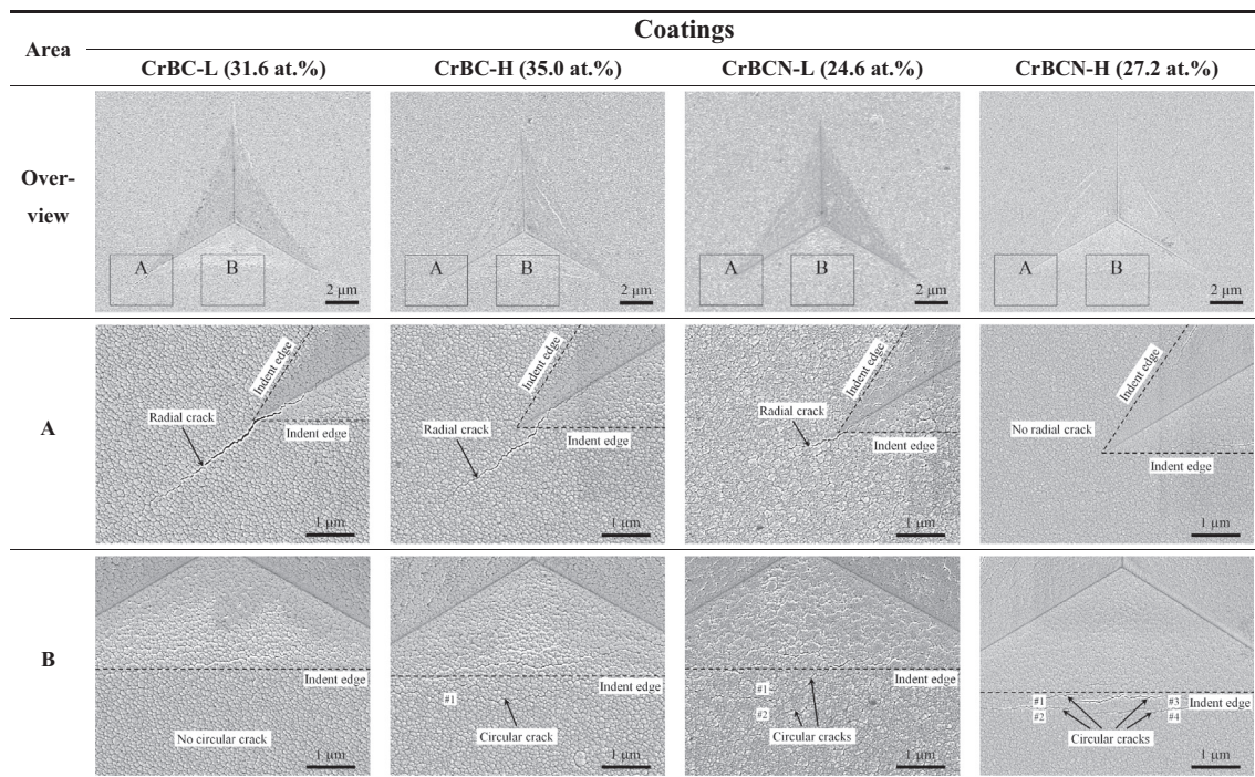
Fig. 5. Overviews and enlarged areas of indent on CrBC and CrBCN coatings with different B concentrations.
