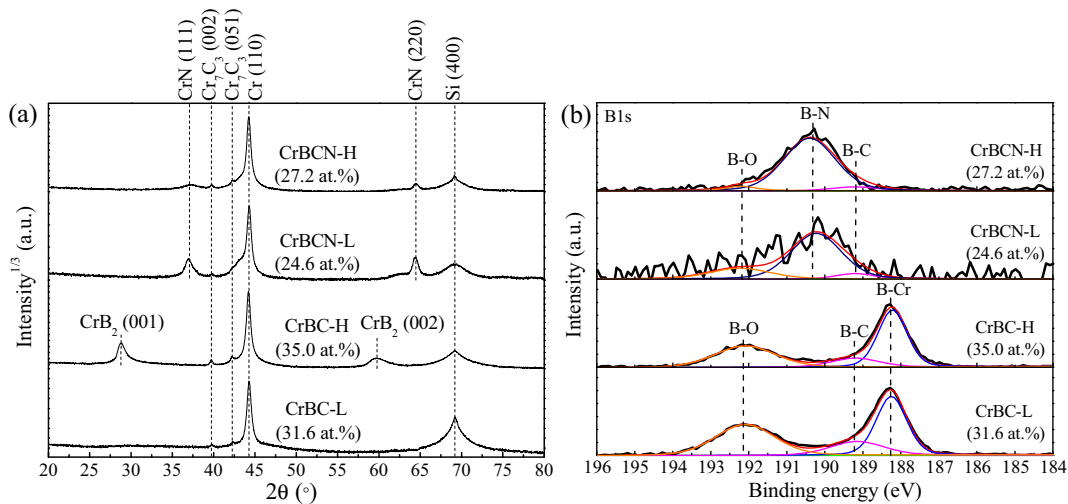
Fig. 2. (a) X-ray diffractograms and (b) B1s XPS spectra of CrBC and CrBCN coatings with different B concentrations.
