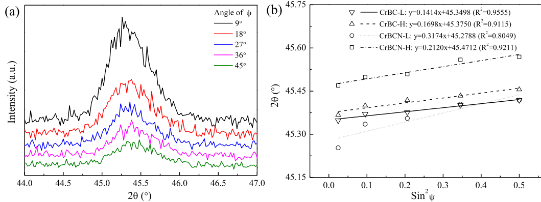
Fig. 1. (a) X-ray diffractograms of CrBC-L coatings at different angles of \psi (b) Liner regressions of CrBC-L, CrBC-H, CrBCN-L and CrBCN-H coatings.
