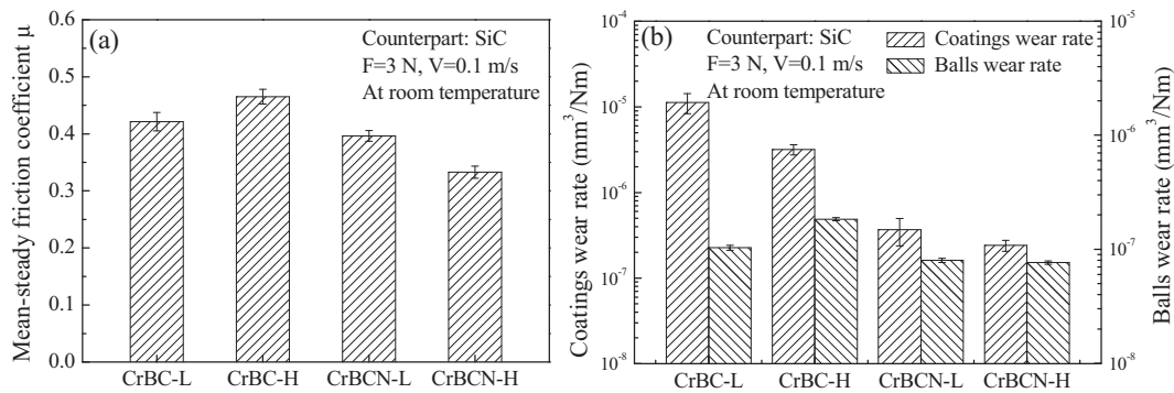
Fig. 7. (a) Mean-steady friction coefficient and (b) wear rates of CrBC/SiC and CrBCN/SiC tribopairs.
