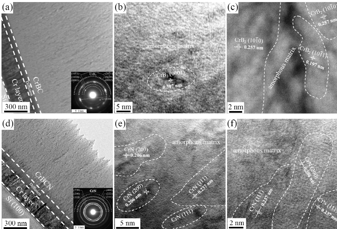
Fig. 4. (a) Cross-sectional morphology with the corresponding SAED and (b) (c) TEM images of CrBC-H coating; (d) cross-sectional morphology with the corresponding SAED and (e) (f) TEM images of CrBCN-L coating.
